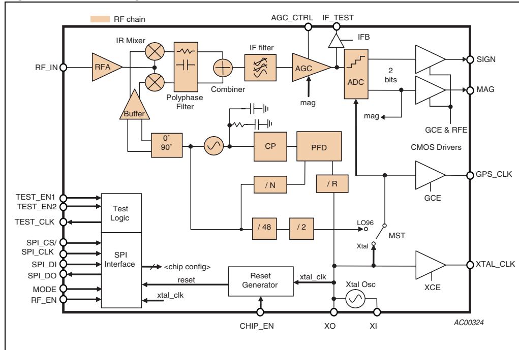
Figure 1. Block diagram
