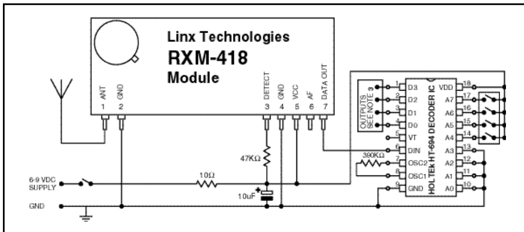
Figure 11: Basic Wireless Decoder circuit
