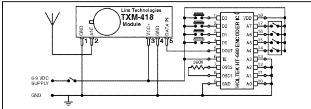
Figure 10: Basic Wireless Encoder circuit
