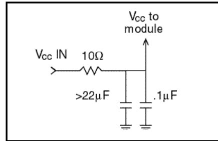
Figure 6: Suggested supply filter
