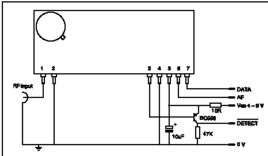
Figure 9: Simple circuit implementing carrier detect
