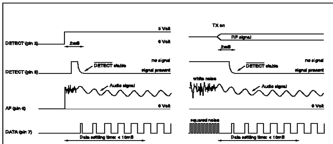
figure 5: Timing Charts
