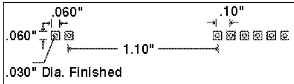
Figure 7: Recommended pad layout
