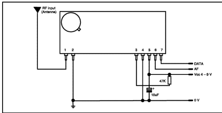
figure 3: Test/Basic application circuit
