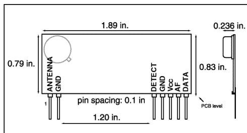
Package Outline
