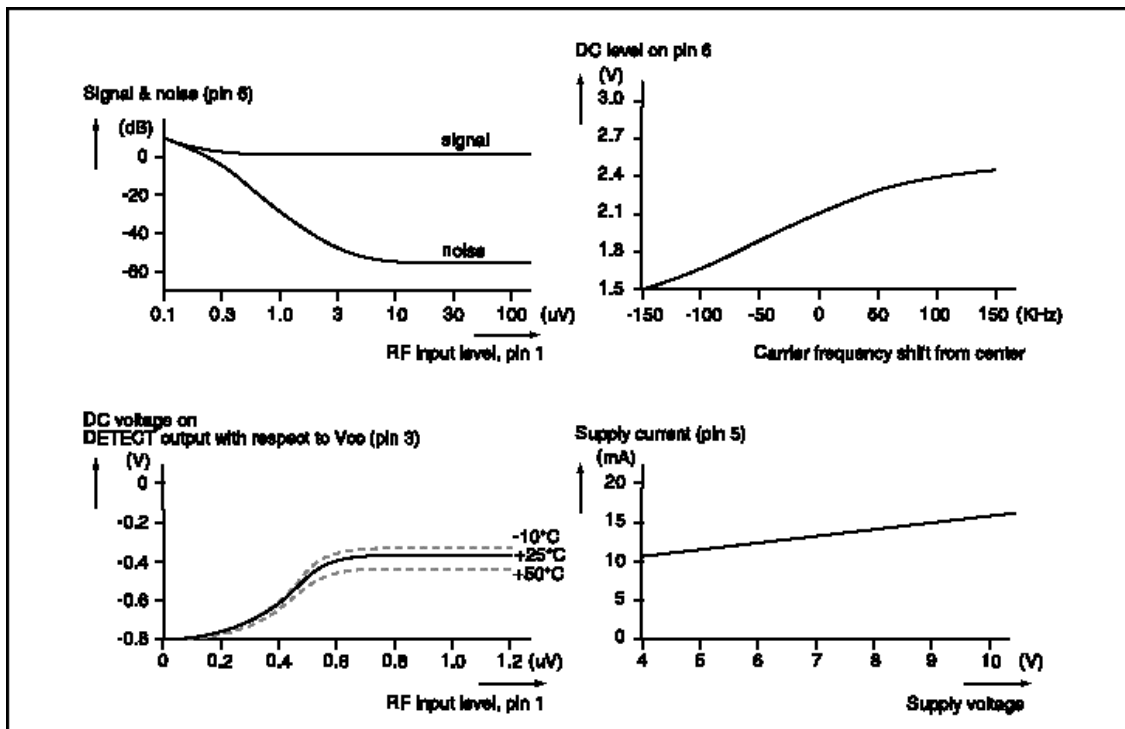
figure 4: Typical performance curves
