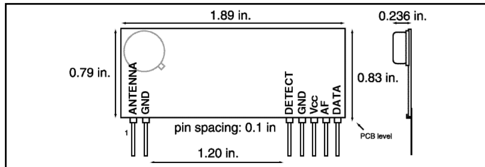
figure 2: mechanical dimensions
