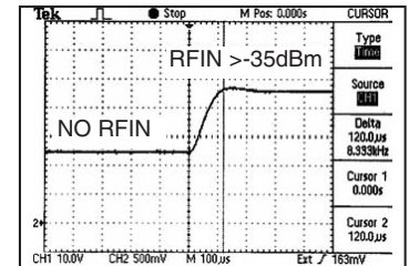
Figure 6: RSSI Response Time
