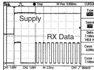
Figure 3: Turn-On Time from V CC
