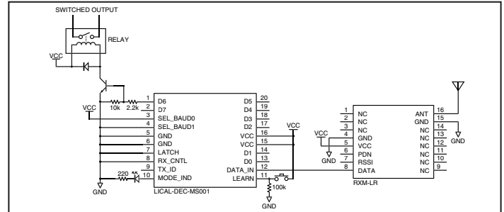
Figure 12: LR Receiver and MS Decoder
