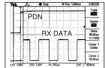
Figure 4: Turn-On Time from PDN
