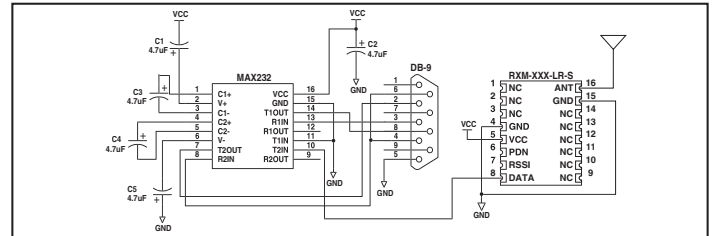
Figure 13: LR Receiver and MAX232 IC
