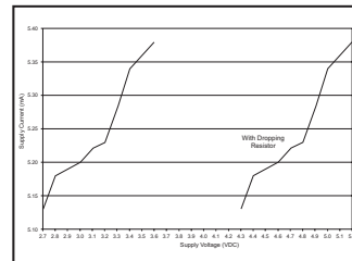
Figure 5: Consumption vs. Supply
