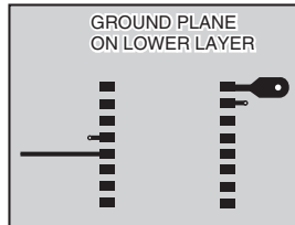
Figure 15: Suggested PCB Layout
