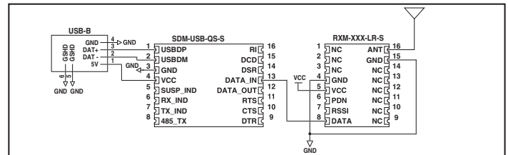
Figure 14: LR Receiver and Linx USB Module
