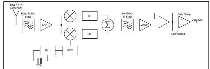
Figure 8: LR Series Receiver Block Diagram
