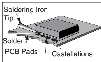
Figure 18: Soldering Technique
