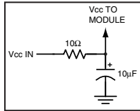
Figure 10: Supply Filter
