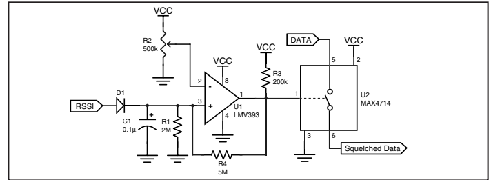
Figure 11: LR Receiver and LS Decoder
