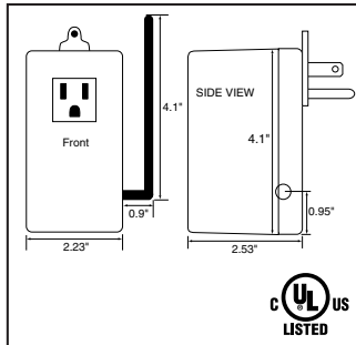
Figure 1: Package Dimensions
