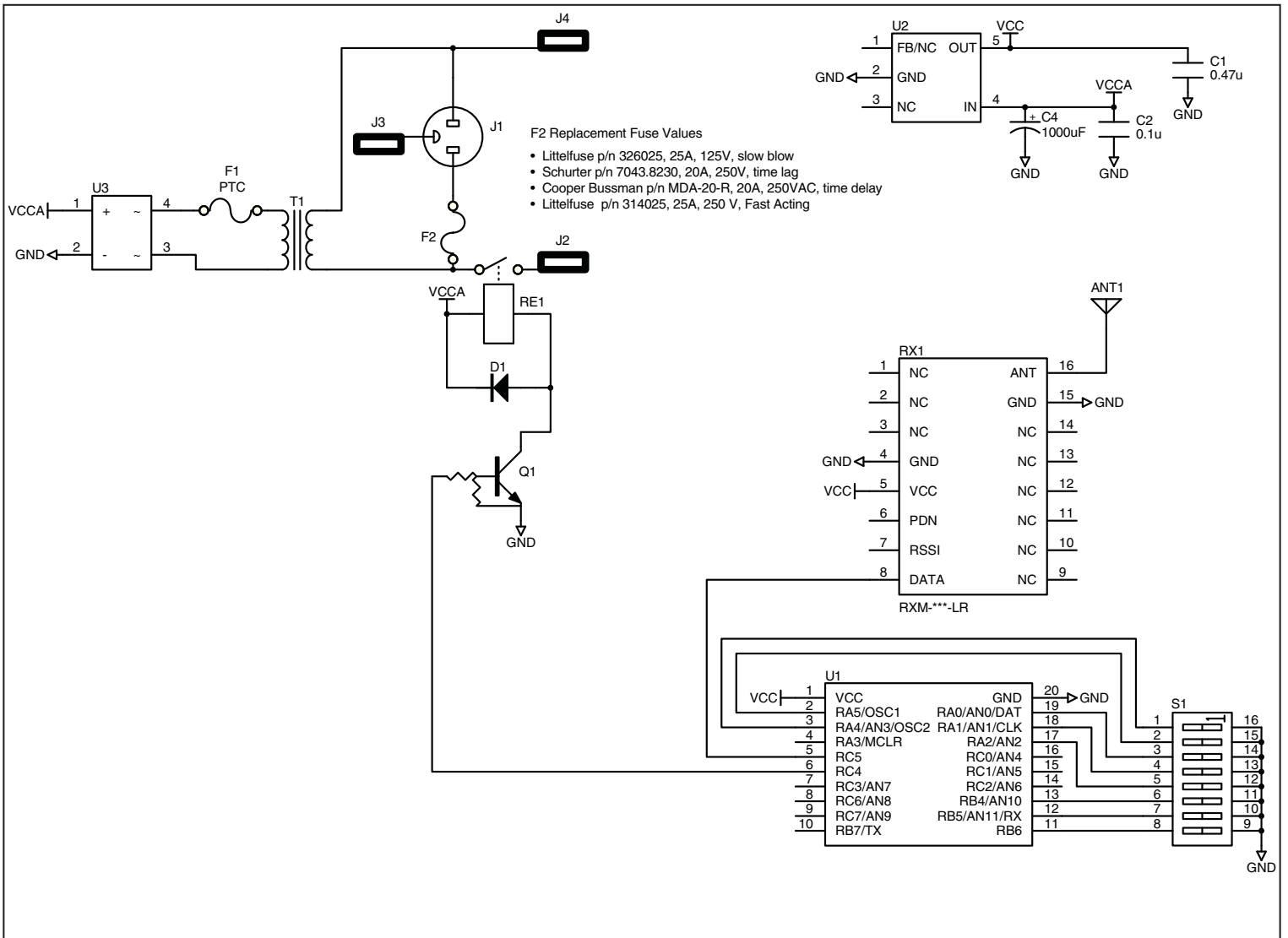
Figure 12: FCTN-WALL-*** Schematic Diagram
