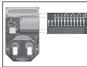
Figure 8: Keyfob Transmitter
