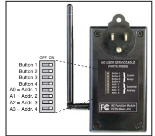
Figure 3: Module DIP Switches
