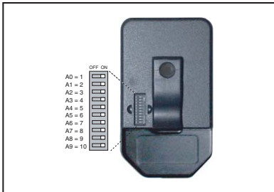
Figure 9: Compact Handheld Transmitter
