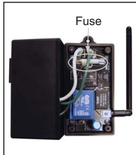
Figure 4: FCTN-WALL-418 Fuse
