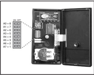
Figure 2: DIP Switch Assignments
