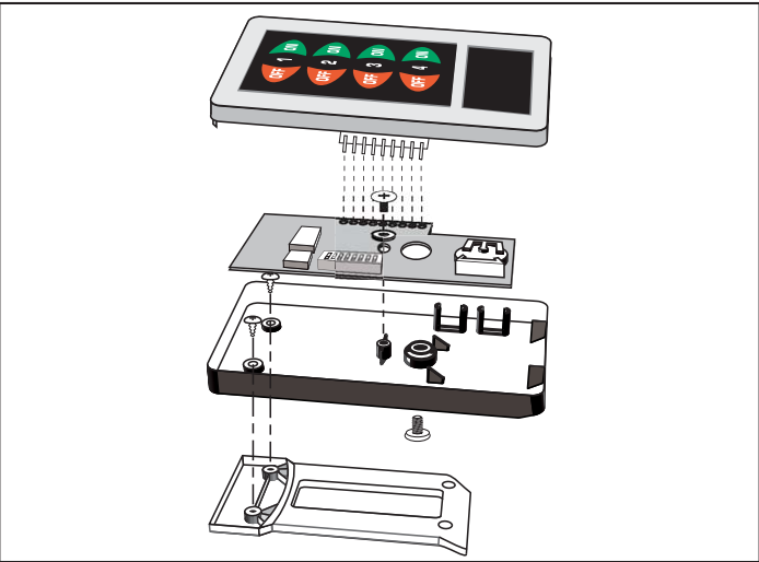
Figure 5: CMD-HHTX-*** Assembly
