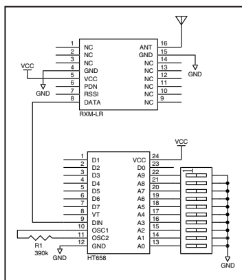
Figure 6: LR Receiver and HT658 Schematic
