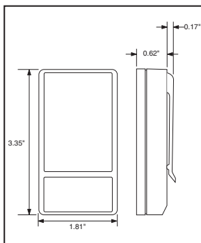
Figure 1: Package Dimensions
