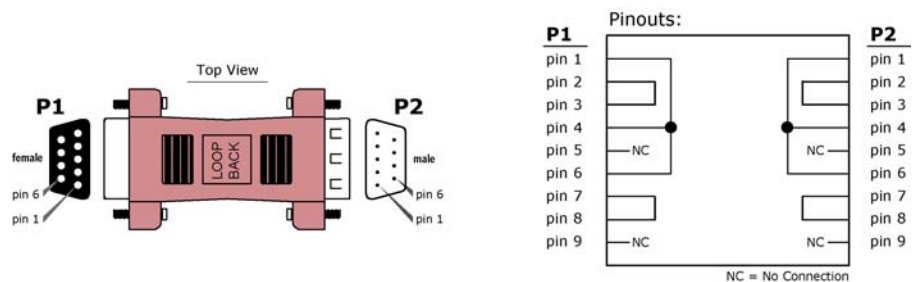
Figure B-04. Serial loopback adapter and pinouts
