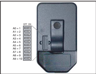
Figure 2: DIP Switch Assignments If the switch is on, the address line is connected to ground, otherwise it is floating. The receiver's address must match exactly in order for the units to communicate. Application Note AN-00300 describes in detail how to set the address to match any of the receivers offered by Linx. This note can be found in the Support section of the Linx website, www.linxtechnologies.com .
