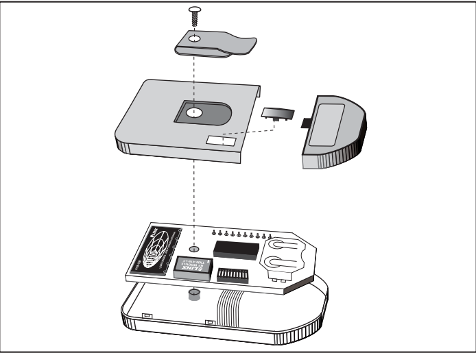
Figure 5: CMD-HHCP-*** Assembly
