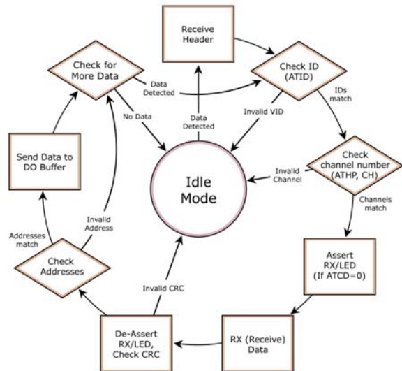
Figure 2-04. Receive Mode Data Flow
