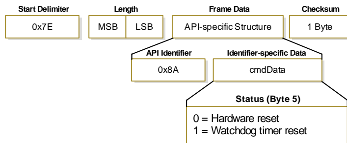
Figure 3-04. RF Modem Status Frames
