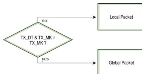
Figure 4-03. Address Recognition (@ the Transmitting RF Modem)
