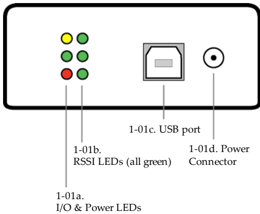
Figure 1-01. Front View
