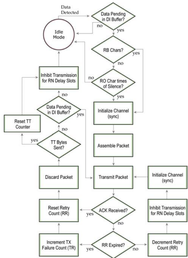
Figure 4-07. Acknowledged Mode State Diagram (TX modem)
