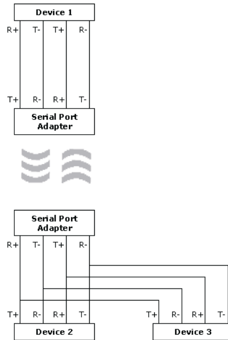
Picture 12. Four-wire RS422 connection setup
