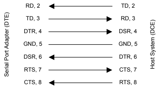
Picture 11. Straight cable
