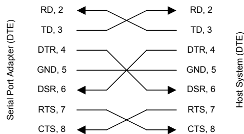
Picture 6. Crossover cable
