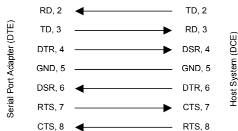
Picture 7. Straight cable
