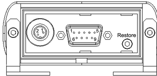
Picture 9. DSUB serial connector (male).
