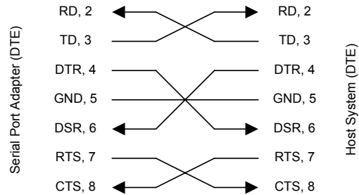
Picture 10. Crossover cable
