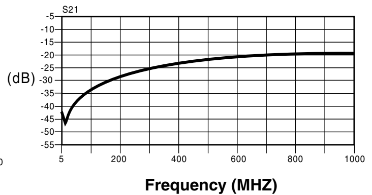
ISOLATION
