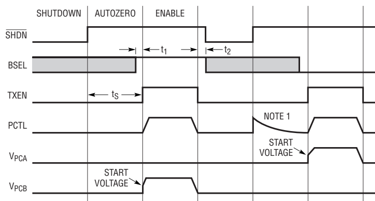
LTC1757A-2 Timing Diagram
