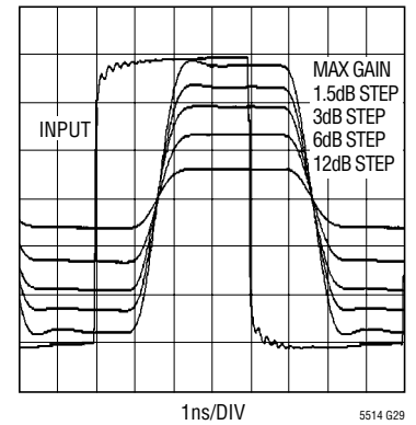
Pulse Response vs Attenuation, Output Level is 4V_{P-P} at Max Gain into 50\Omega External Load
