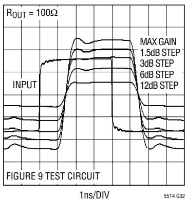
Pulse Response vs Attenuation, LT5514 Levels are: V_{IN} = 66mV_{P-P} , V_{OUT} = 2V_{P-P} at Max Gain
