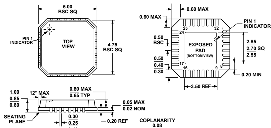
COMPLIANT TO JEDEC STANDARDS MO-220-VHHD-2 Figure 77. 32-Lead Lead Frame Chip Scale Package [LFCSP_VQ] 5 mm × 5 mm Body, Very Thin Quad Lead (CP-32-8) Dimensions shown in millimeters
