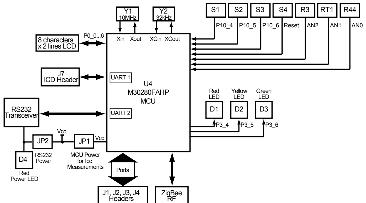
Figure 5-2: RZB-CC16C-ZDK Block Diagram
