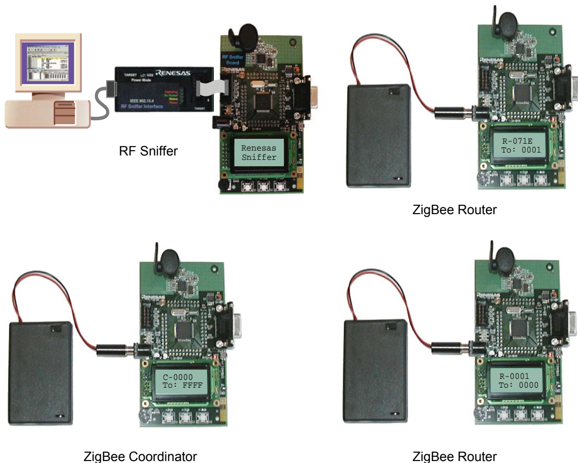
Figure 4-1: ZigBee Demo Kit Setup
