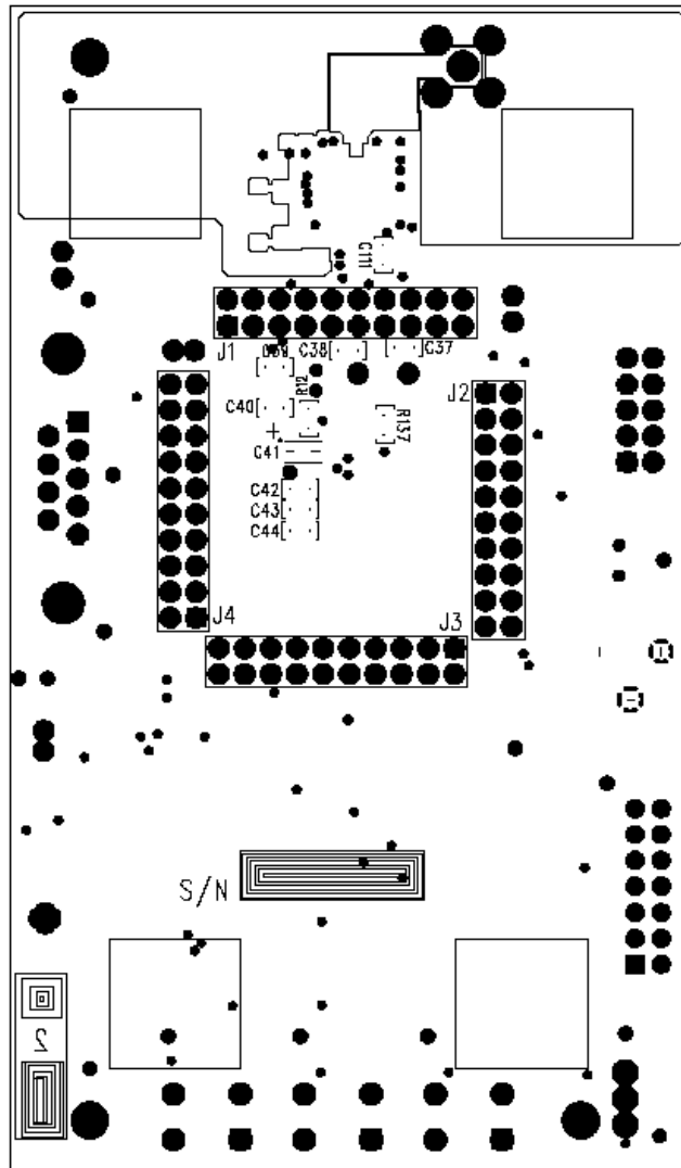
Figure E-2: PCB Bottom View
