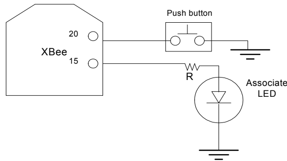
Figure 5-020. Commissioning Pushbutton and Associate LED Functionalities
