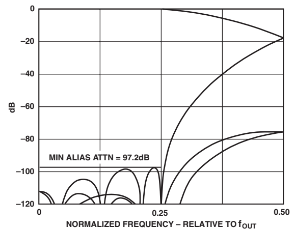
Figure 17b. Folded Decimator Frequency Response for K = 1
