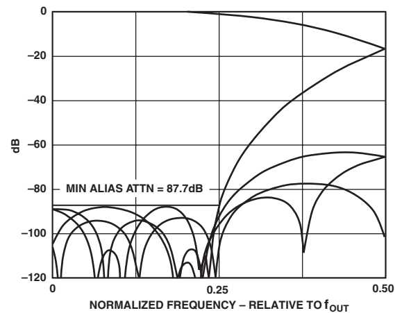
Figure 17a. Folded Decimator Frequency Response for K = 0
