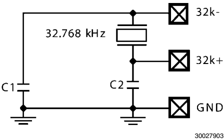
FIGURE 4. 32.768 kHz Oscillator
