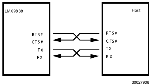
FIGURE 7. UART NULL Modem Connection
