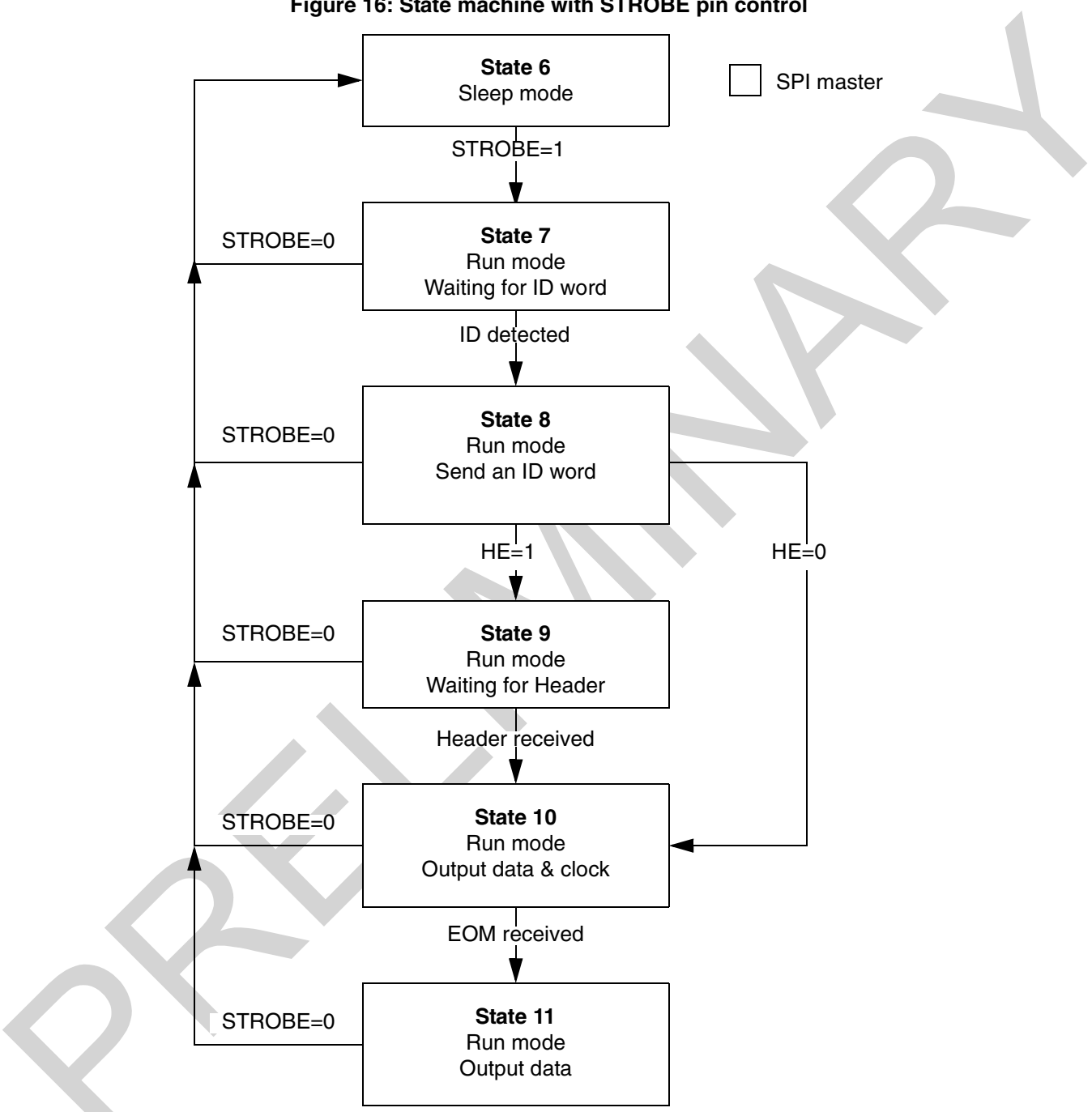
Figure 16: State machine with STROBE pin control
