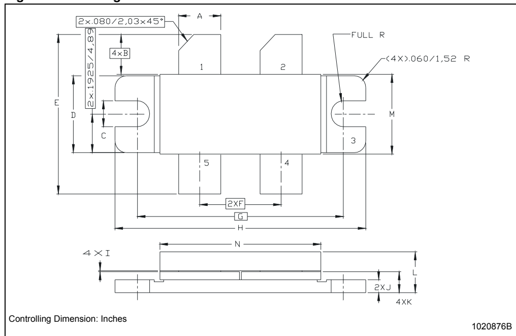
Figure 6. Package dimensions
