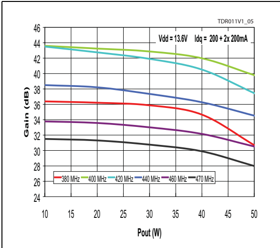
Figure 5. Gain vs. output power
