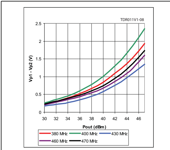
Figure 7. Vp1-Vp2 vs. output power
