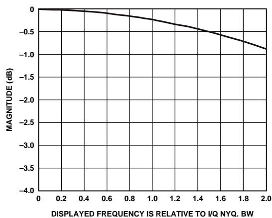
Figure 42. Pass-Band Detail (R = 63, HBF 3 Active)
