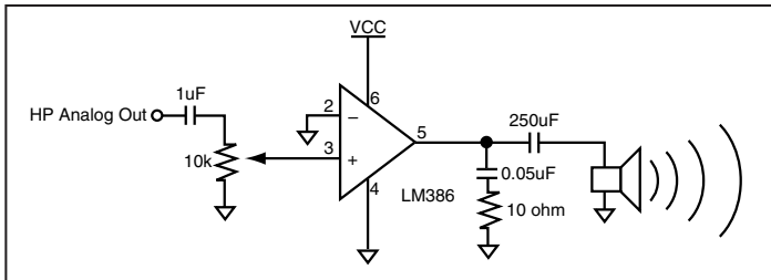
Figure 12: Audio Buffer Amplifier
