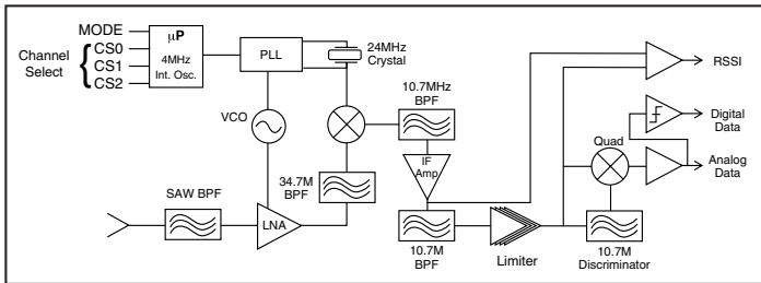
Figure 9: HP3 Series Receiver Block Diagram
