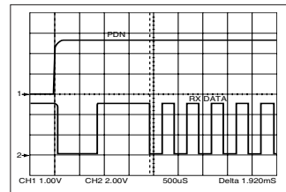
Figure 3: RX Enabled to Valid Data
