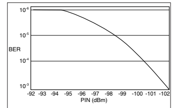
Figure 6: BER vs. Input Power (typical)
