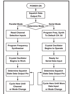
Figure 10: Start-Up Sequence
