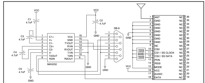
Figure 14: HP3 Receiver and MAX232 IC
