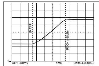
Figure 5: Worst Case RSSI Response Time
