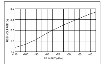
Figure 4: Receiver RSSI
