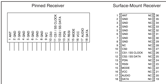
Figure 7: HP3 Series Receiver Pinout
