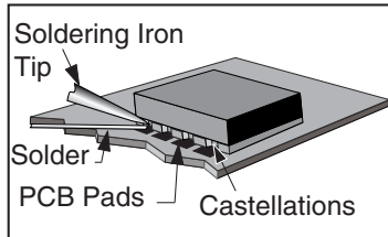
Figure 8: Soldering Technique
