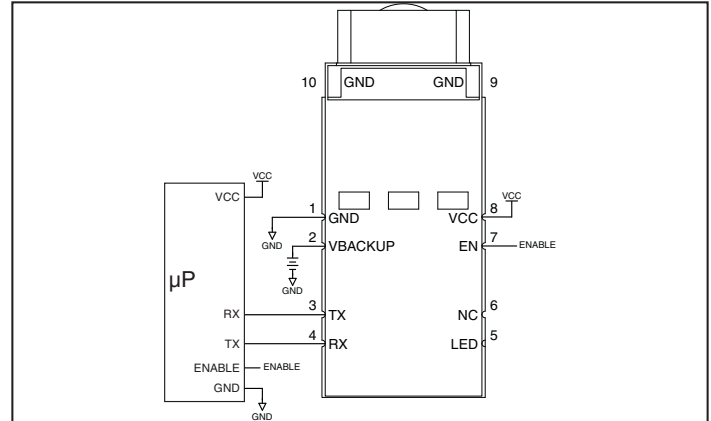
Figure 3: SR Series Module Typical Application
