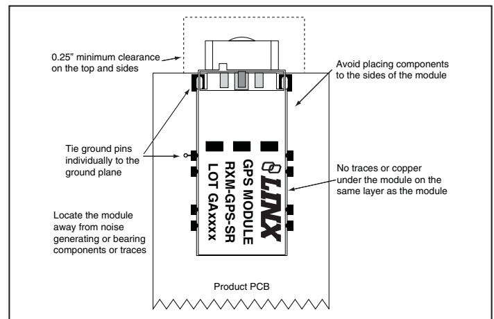
Figure 6: Antenna Considerations
