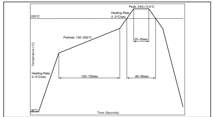
Figure 9: Maximum Reflow Profile
