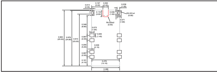
Figure 7: Recommended PCB Layout
