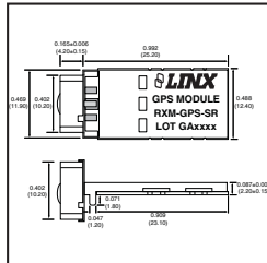
Figure 1: Package Dimensions
