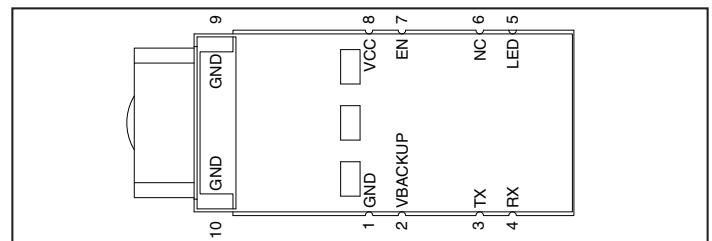
Figure 2: SR Series Receiver Pinout (Top View)
