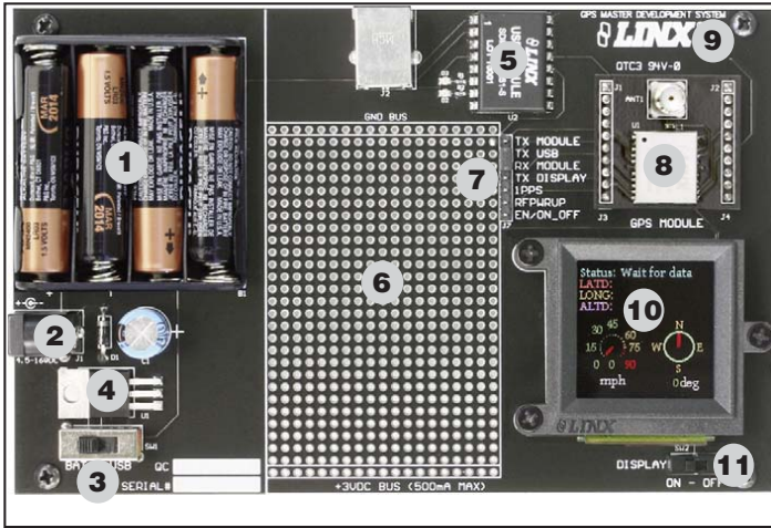
Figure 1: SG Series Receiver Development Board
