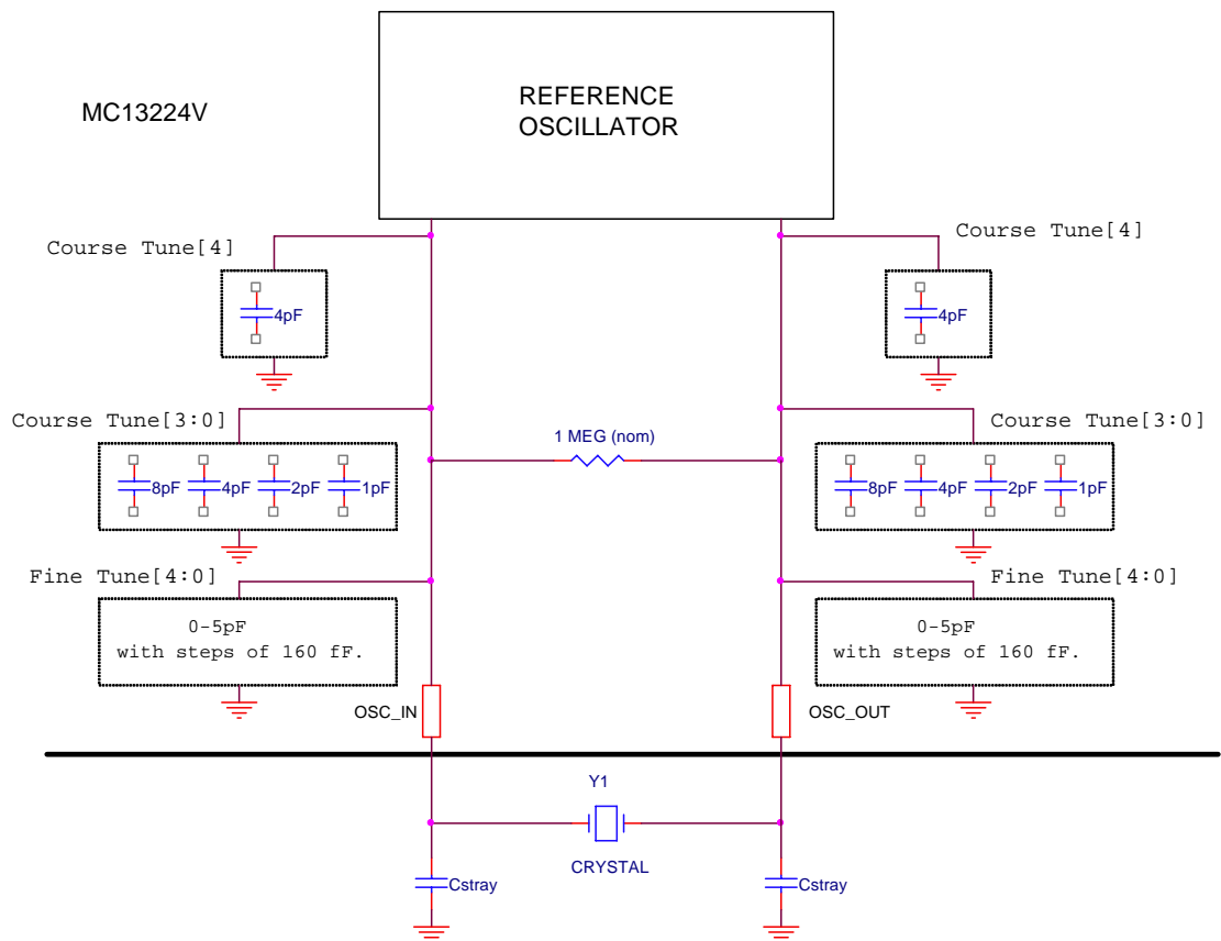
Figure 10. Reference Oscillator Model
