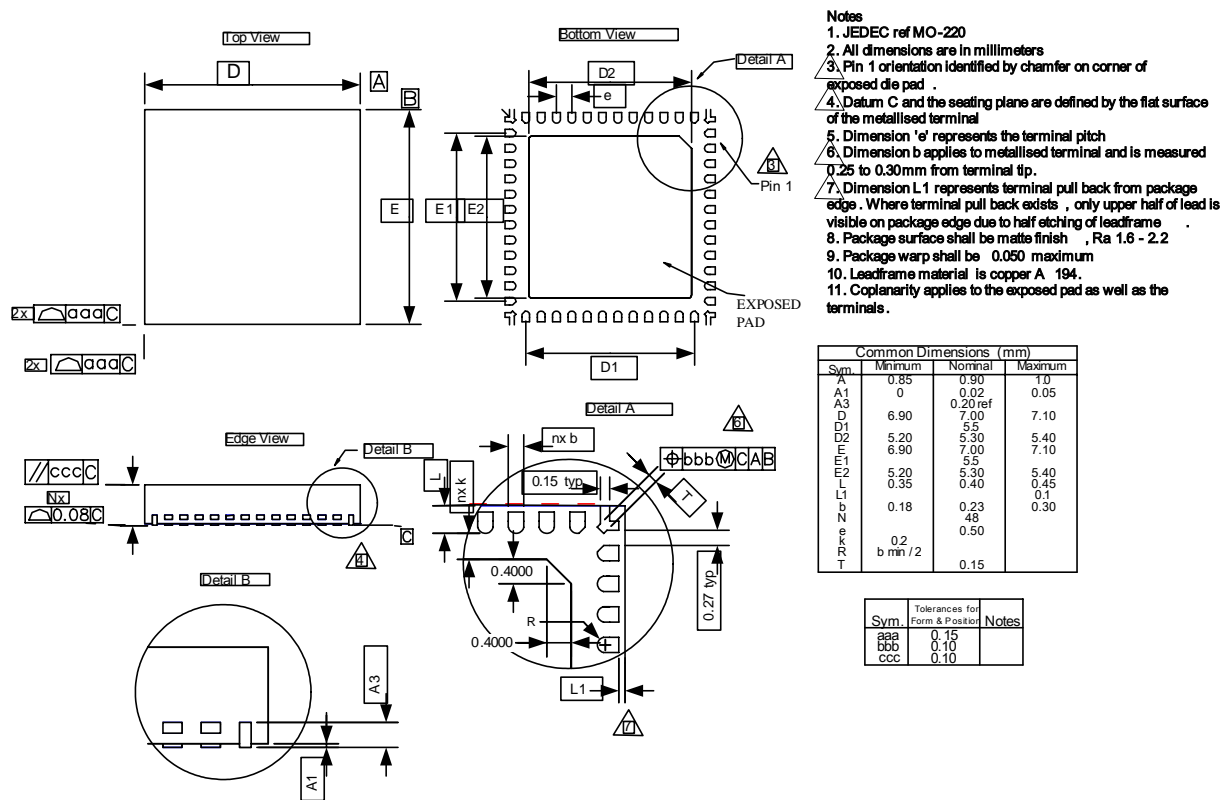
Figure 17. Package Drawing
