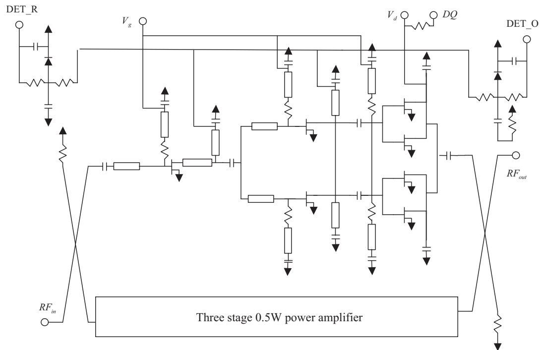
Figure 11. AMMC-6440 Schematic
