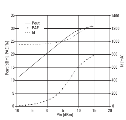
Figure 6. Typical Output Power, PAE, and Total Drain Current versus Input Power at 24GHz
