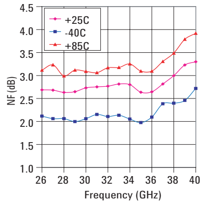
Figure 11. Noise Figure Over Temperature
