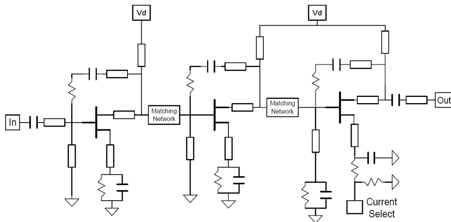
Figure 21. Simplified High Linearity LNA Schematic
