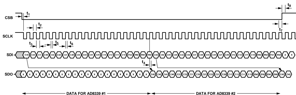
Figure 57. Timing Diagram
