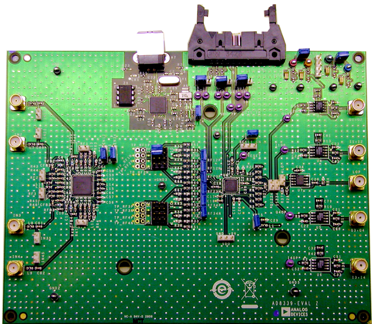
Figure 58. AD8339 Evaluation Board
