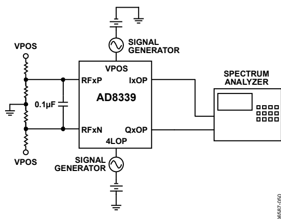
Figure 51. PSRR
