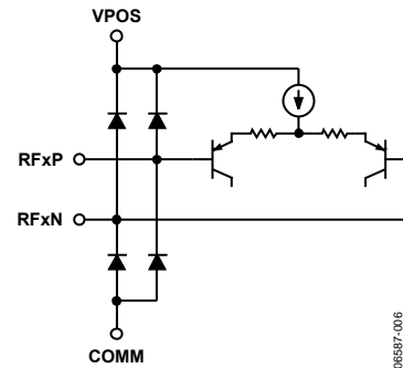
Figure 7. RF Inputs
