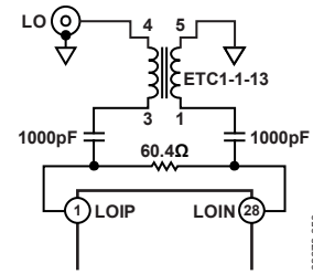
Figure 50. Differential LO Drive with Balun
