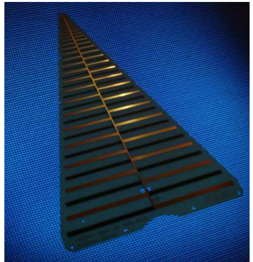
Gold-coated, protected TEFLON precision antenna
