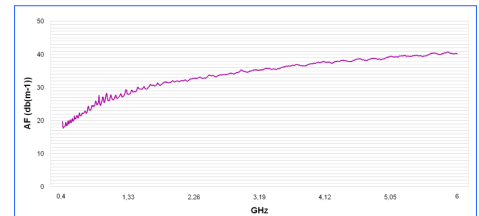
Antenna factor HyperLOG 4060
