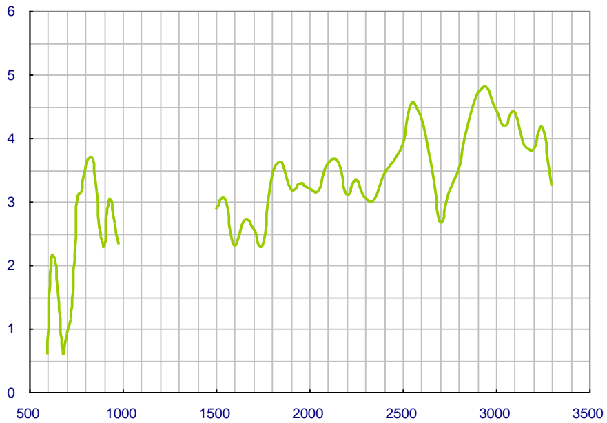
Antena Gain of FXP.400 with 200mm ground
