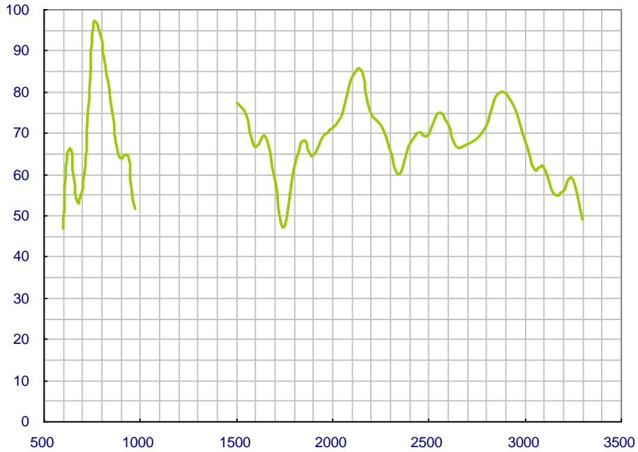
Antenna Efficiency of FXP.400 with 200mm ground
