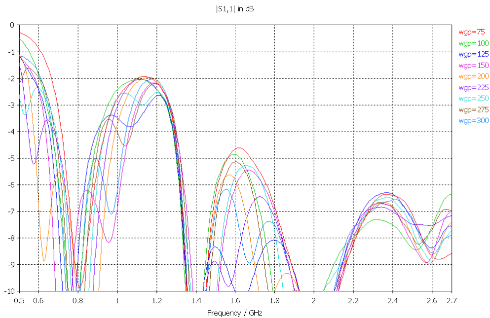
wgp = Ground plane width (mm)
