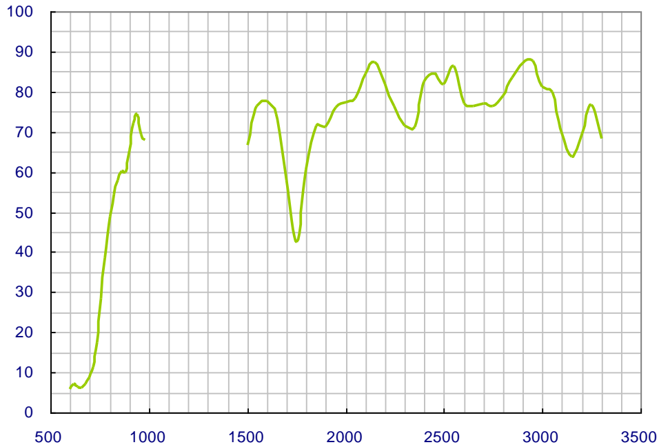
Antenna Efficiency of FXP.400 with 100mm Ground
