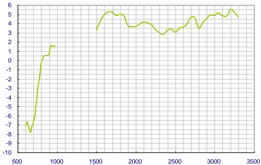
Antenna Gain of FXP.400 with 80mm Ground
