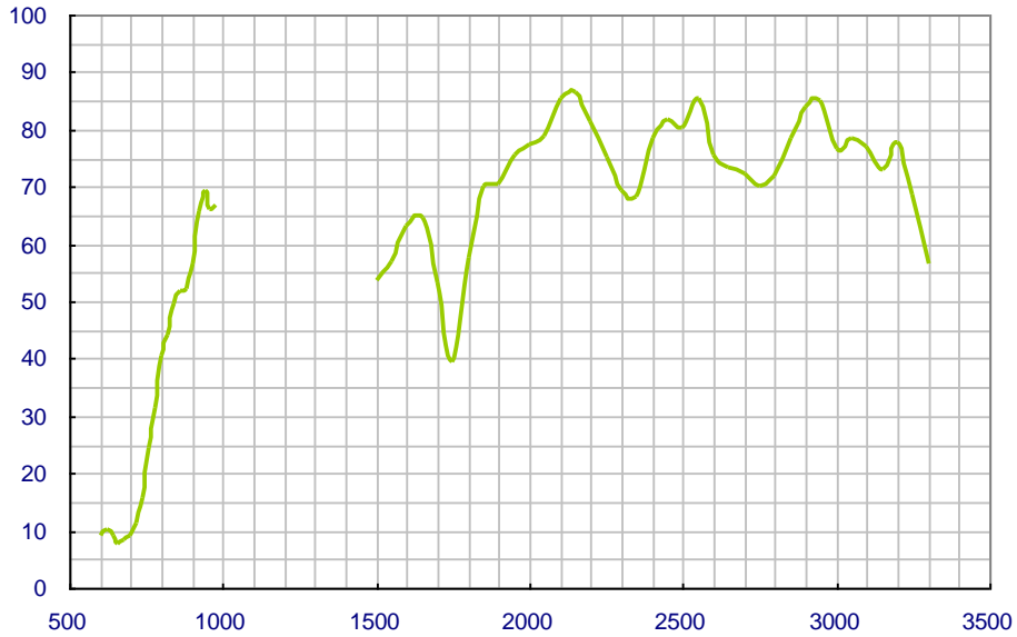
Antenna Efficiency of FXP.400 with 80mm Ground
