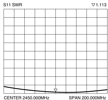
Typical VSWR
