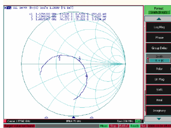
Smith Chart
