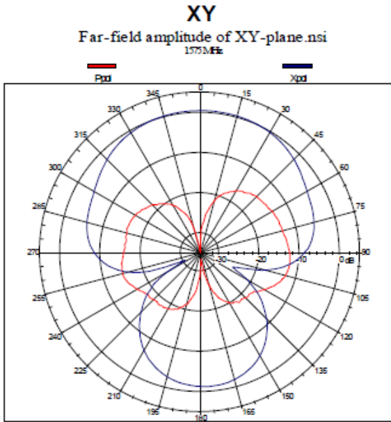
Linear polarized signal f_0=1575.42\text{MHz}
