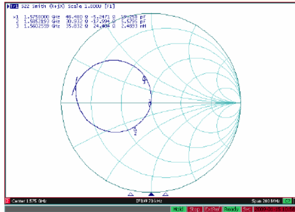
Smith Chart
