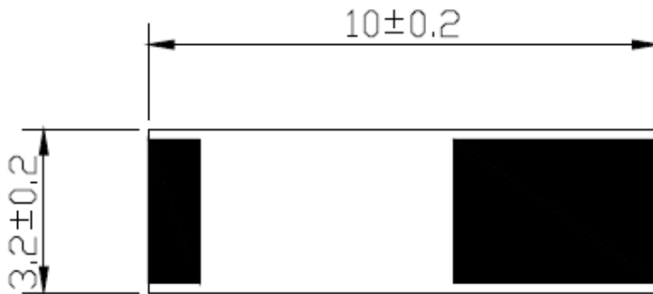
Vertical View
