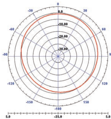
ZY-Plane ( \phi = 90 )
