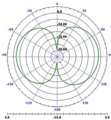
XY-Plane ( \theta = 90 )
