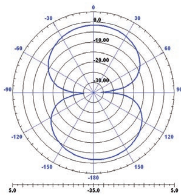
ZX-Plane ( \phi = 0 )
