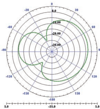
XY-Plane ( \theta = 90 )
