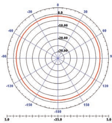
ZY-Plane ( \phi = 90 )
