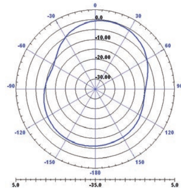
ZX-Plane ( \phi = 0 )
