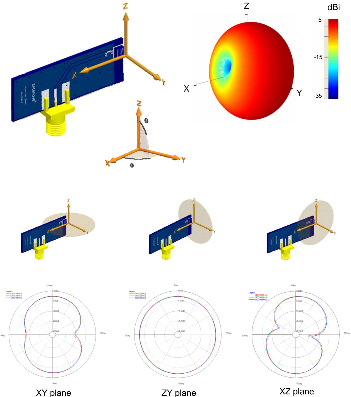
Patterns show combined polarisations measured on reference board A10192-U1
