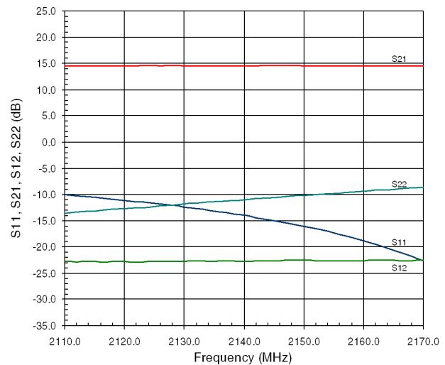
RF3807415 Evaluation Board S-Parameters
