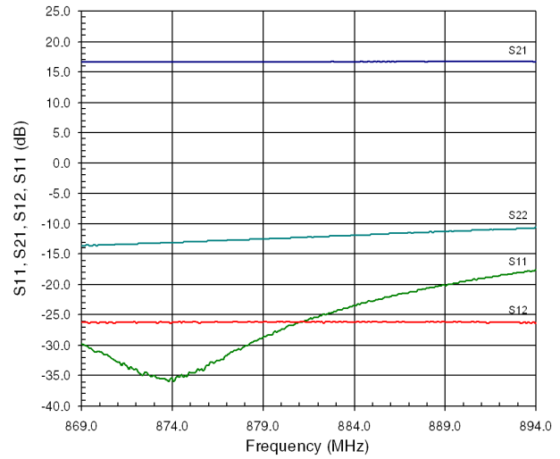
RF3807413 Evaluation Board S-Parameters
