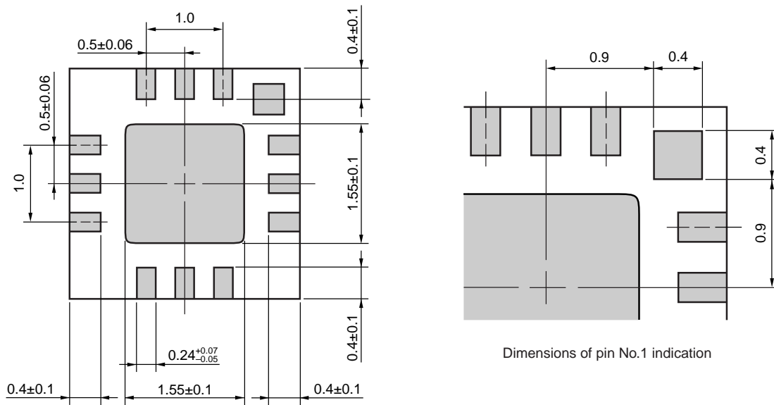
(Bottom View)
