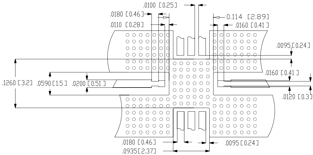
Figure 16a. PCB Land Pattern
