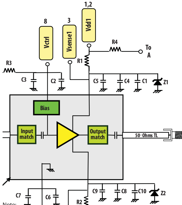
Note: To supply Vdd1 and Vdd2 individually, remove R4 and supply Vdd1 from pin 1,2 and Vdd2 from pin 19,20
