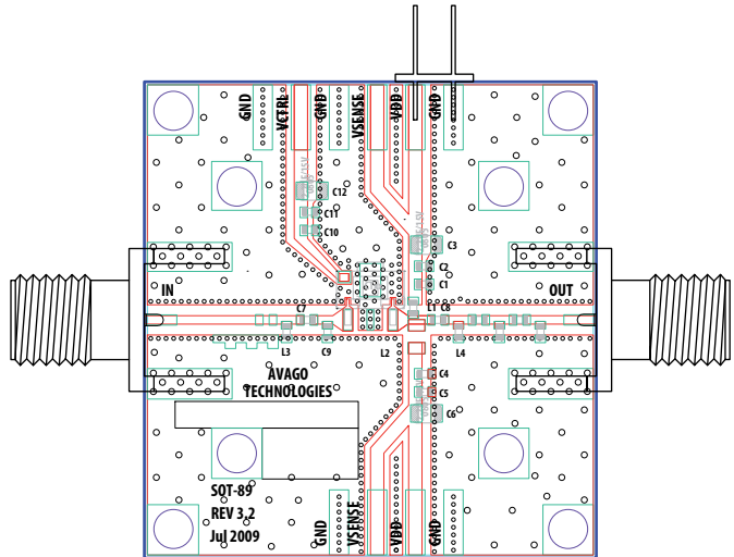
Figure 35. Demoboard
