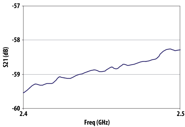
Figure 9e. Rejection plot for WLAN band @ Vdd = 2.7V, Idd = 7.5mA
