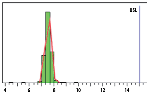
Figure 3. I d at 1.575 GHz; USL = 15 mA, nominal = 7.5 mA
