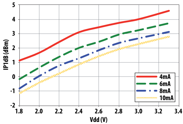
Figure 24. IP1dB vs. Vdd at 25°C
