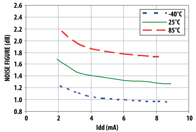
Figure 15. NF vs Idd at Vdd = 1.8V
