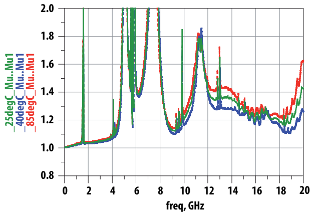
Figure 26. Edwards-Sinsky Output Stability Factor ( \mu ) at V_{dd} = 2.7V
