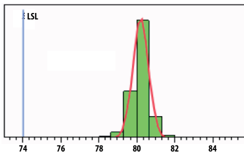
Figure 5. PCS band Rejection at 1850MHz relative to 1.575 GHz; LSL = 74 dBc, nominal = 80.2 dBc
