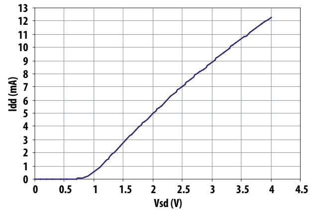
Figure 12. I_{dd} vs V_{sd} for V_{dd} = 2.7V , R_2 = 6.8k \text{ Ohm}
