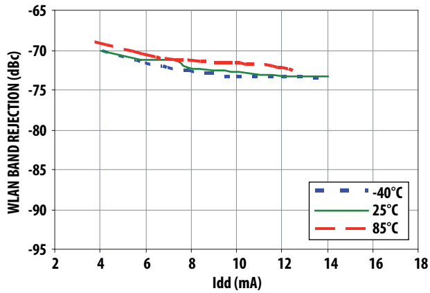
Figure 22. WLAN band rejection vs. Idd at Vdd = 2.7V
