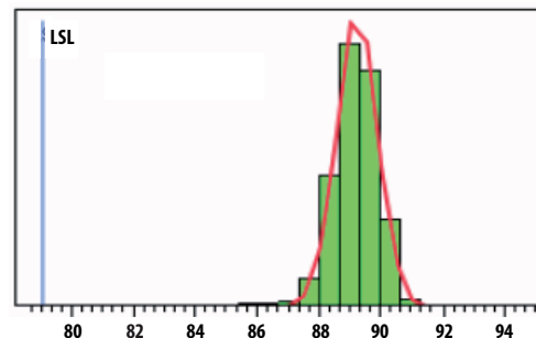
Figure 4. Cell band Rejection at 928MHz relative to 1.575 GHz; LSL = 79 dBc, nominal = 89.2 dBc
