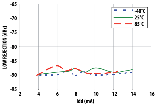
Figure 18. Low band rejection vs. Idd at Vdd = 2.7V
