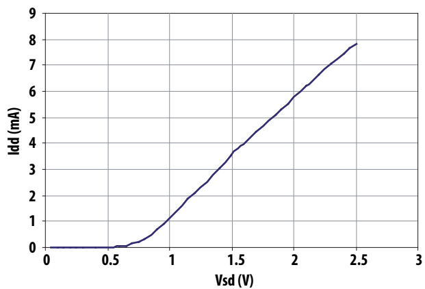
Figure 13. I_{dd} vs V_{sd} for V_{dd} = 1.8V , R_2 = 2.7k \text{ Ohm}
