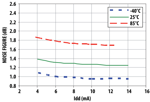
Figure 14. NF vs. Idd at Vdd = 2.7V
