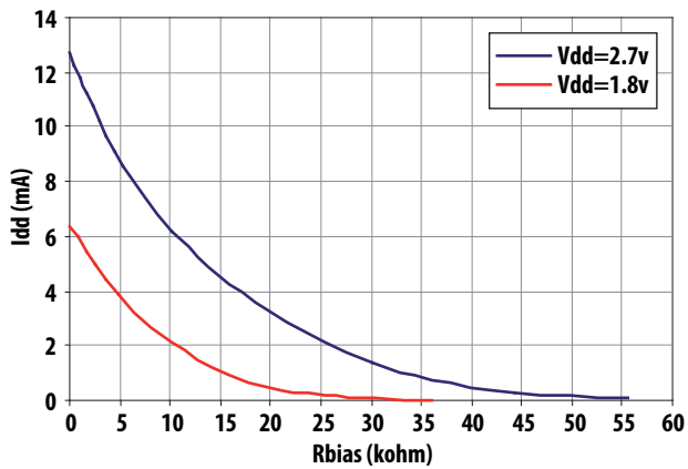
Figure 11. I_{dd} vs R_{bias} at 25°C
