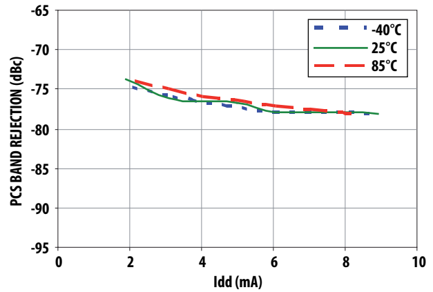
Figure 21. High band rejection vs. Idd at Vdd = 1.8V
