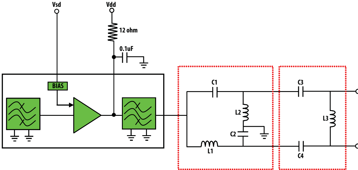
Figure 30. Proposed Balun design for ALM-2712
