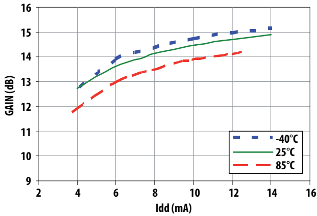
Figure 16. Gain vs. Idd at Vdd = 2.7V
