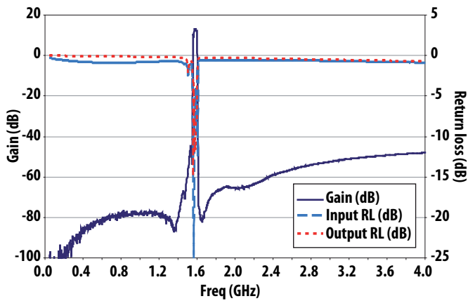
Figure 10a. Typical S-Parameter Plot @ V_{dd} = 1.8V , I_{dd} = 5mA
