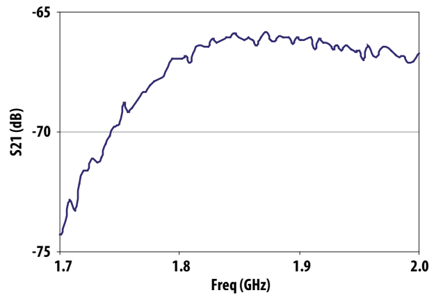
Figure 9d. Rejection plot for High band @ Vdd = 2.7V, Idd = 7.5mA
