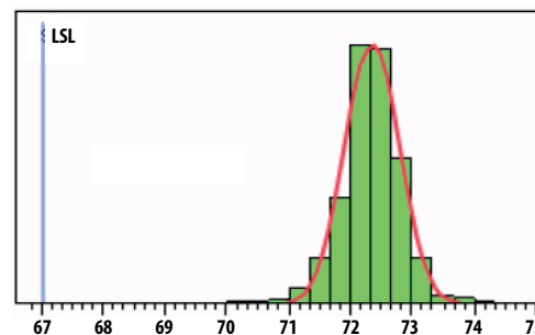
Figure 6. WLAN band Rejection at 2500MHz relative to 1.575 GHz; LSL = 67 dBc, nominal = 72.3 dBc
