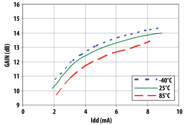
Figure 17. Gain vs. Idd at Vdd = 1.8V
