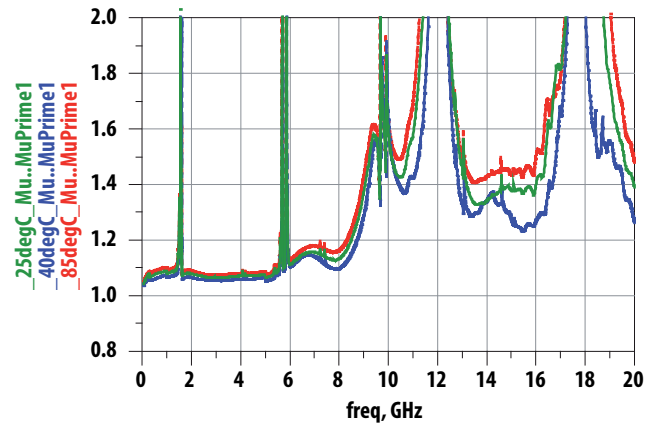
Figure 27. Edwards-Sinsky Input Stability Factor ( \mu' ) at V_{dd} = 2.7V
