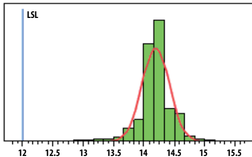
Figure 1. Gain at 1.575 GHz; LSL = 12 dB, nominal = 14.2 dB
