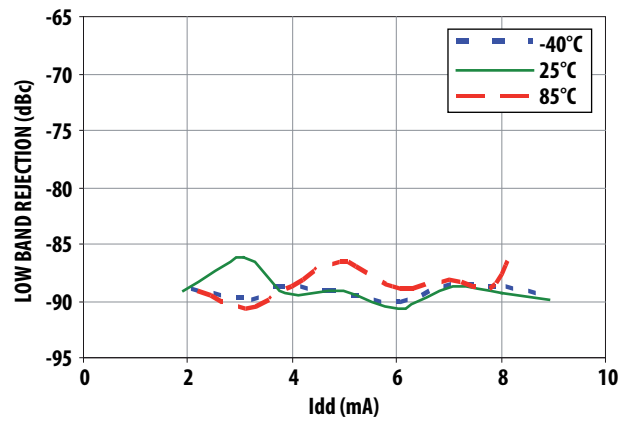
Figure 19. Low band rejection vs. Idd at Vdd = 1.8V
