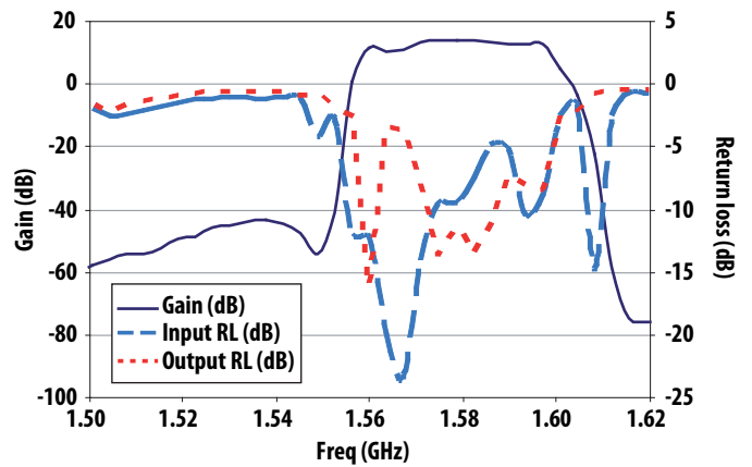
Figure 9b. Passband response of typical S-Parameter Plot @ Vdd = 2.7V, Idd = 7.5mA
