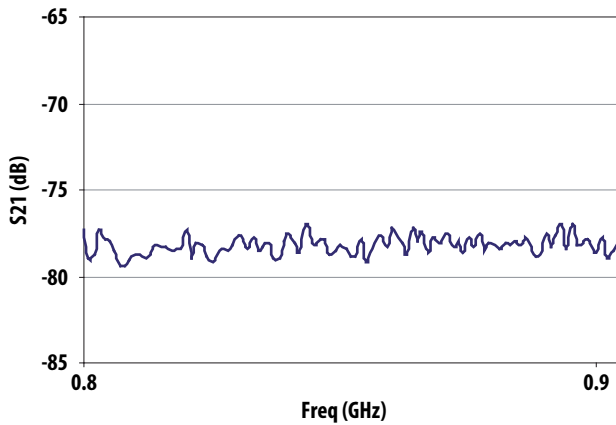
Figure 9c. Rejection plot for Low band @ Vdd = 2.7V, Idd = 7.5mA
