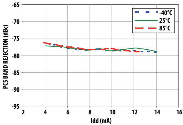
Figure 20. High band rejection vs. Idd at Vdd = 2.7V
