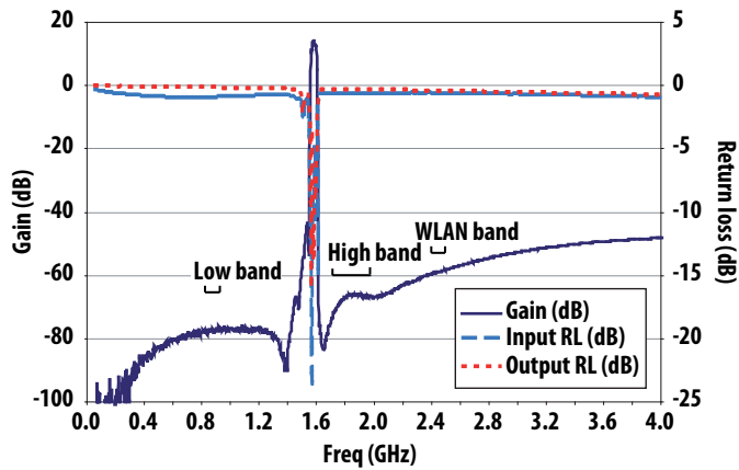
Figure 9a. Typical S-Parameter Plot @ Vdd = 2.7V, Idd = 7.5mA
