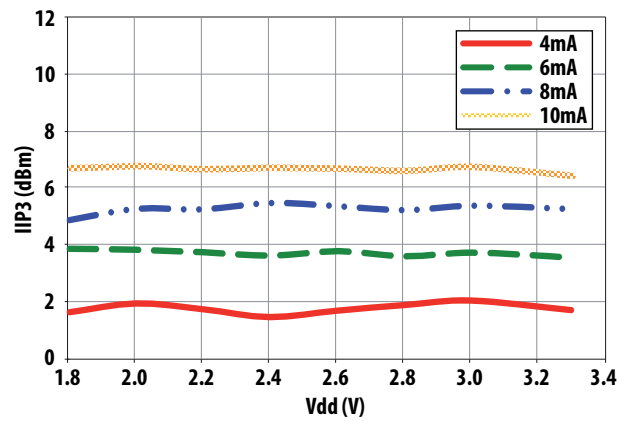
Figure 25. IIP3 vs. Vdd at 25°C
