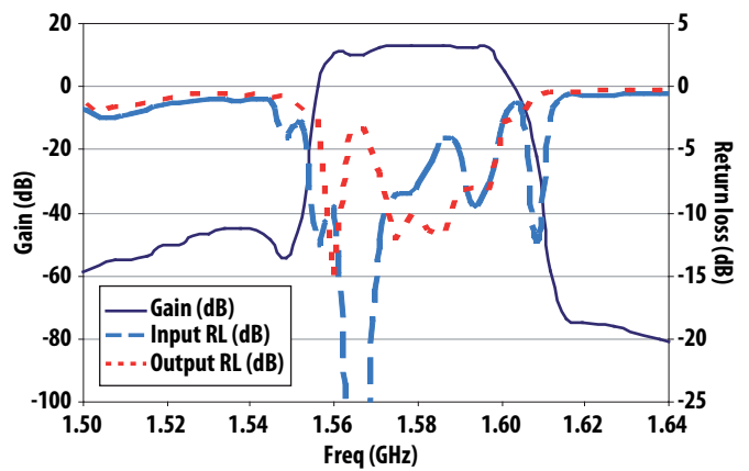
Figure 10b. Passband response of typical S-Parameter Plot @ V_{dd} = 1.8V , I_{dd} = 5mA
