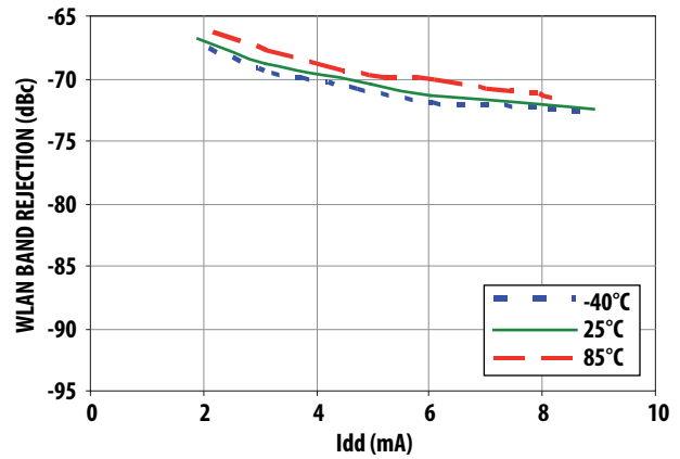
Figure 23. WLAN band rejection vs. Idd at Vdd = 1.8V
