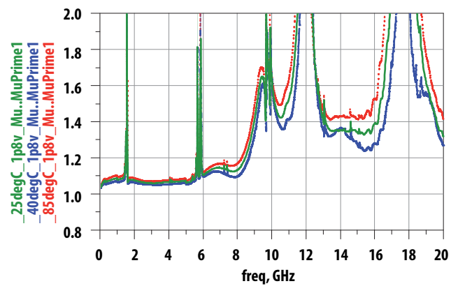
Figure 29. Edwards-Sinsky Input Stability Factor ( \mu' ) at V_{dd} = 1.8V
