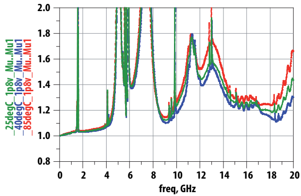
Figure 28. Edwards-Sinsky Output Stability Factor ( \mu ) at V_{dd} = 1.8V
