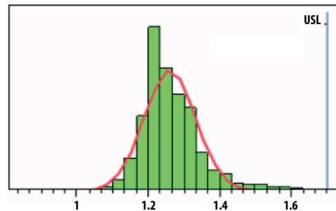
Figure 2. NF at 1.575GHz; USL = 1.7 dB, nominal = 1.26 dB
