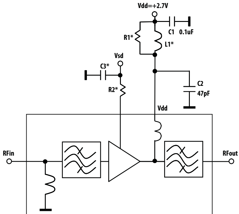
Figure 8. Application Circuit
