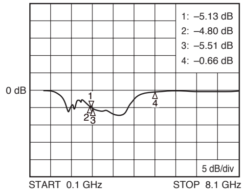
S 22 -FREQUENCY
