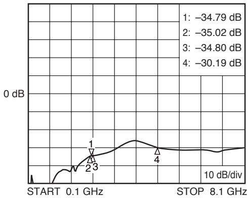
S 12 -FREQUENCY
