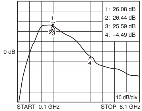
S 21 -FREQUENCY
