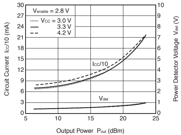
CIRCUIT CURRENT, V det , vs. OUTPUT POWER
