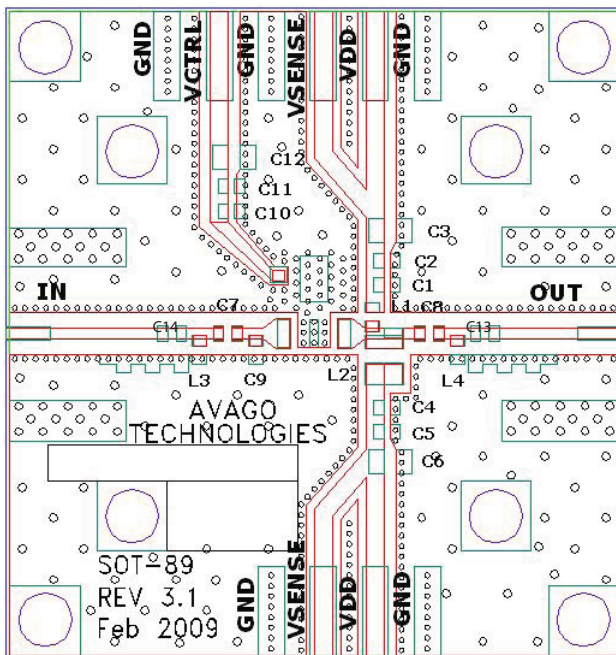
Figure 23. Demo board Layout
