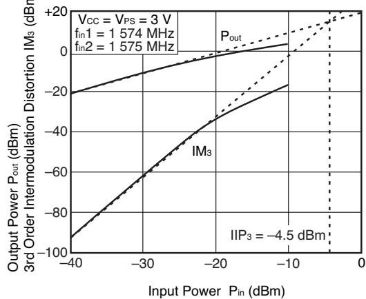
OUTPUT POWER, IM3 vs. INPUT POWER
