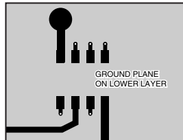
Figure 7: Suggested PCB Layout
