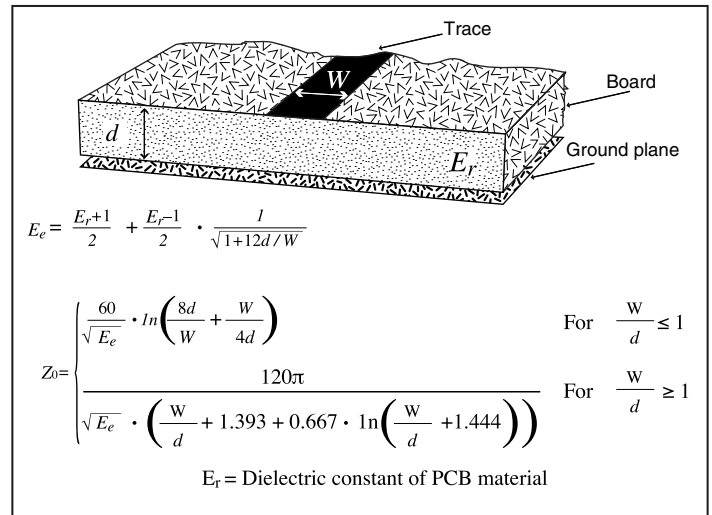
Figure 8: Microstrip Formulas
