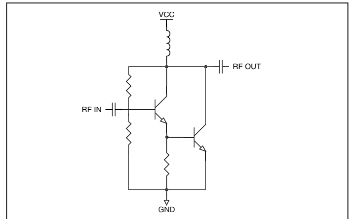
Figure 4: BBA Series Amplifier Schematic
