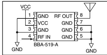
Figure 2: Test / Basic Application Circuit
