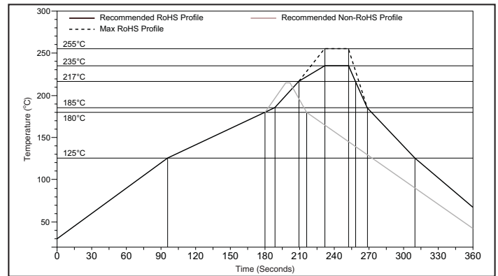
Figure 11: Maximum Reflow Profile
