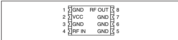
Figure 3: BBA Series Amplifier Pinout (Top View)
