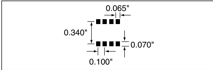
Figure 9: Recommended PCB Layout
