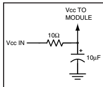
Figure 5: Supply Filter
