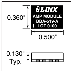
Figure 1: BBA Package Dimensions
