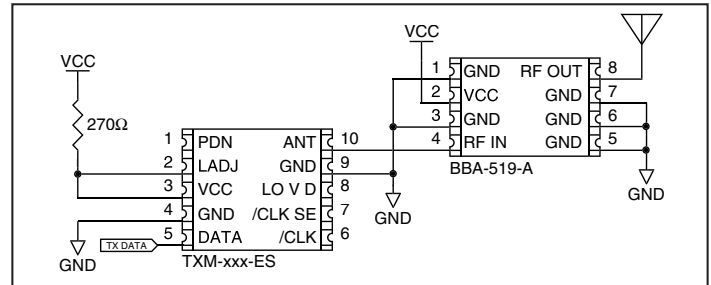
Figure 6: Typical Application Circuit
