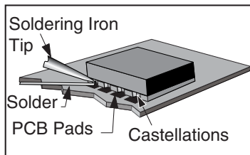
Figure 10: Soldering Technique
